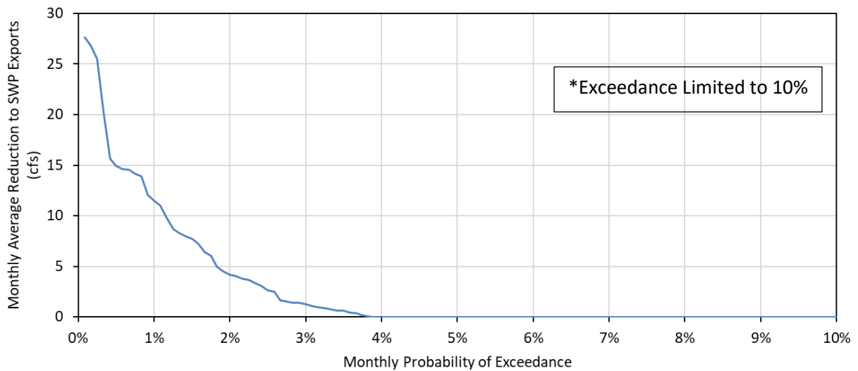
Figure 11. Monthly Probability of Exceedance (1,200 months) of Potential Reduction to SWP Exports from Changed Del Puerto Creek Flow [PA]
