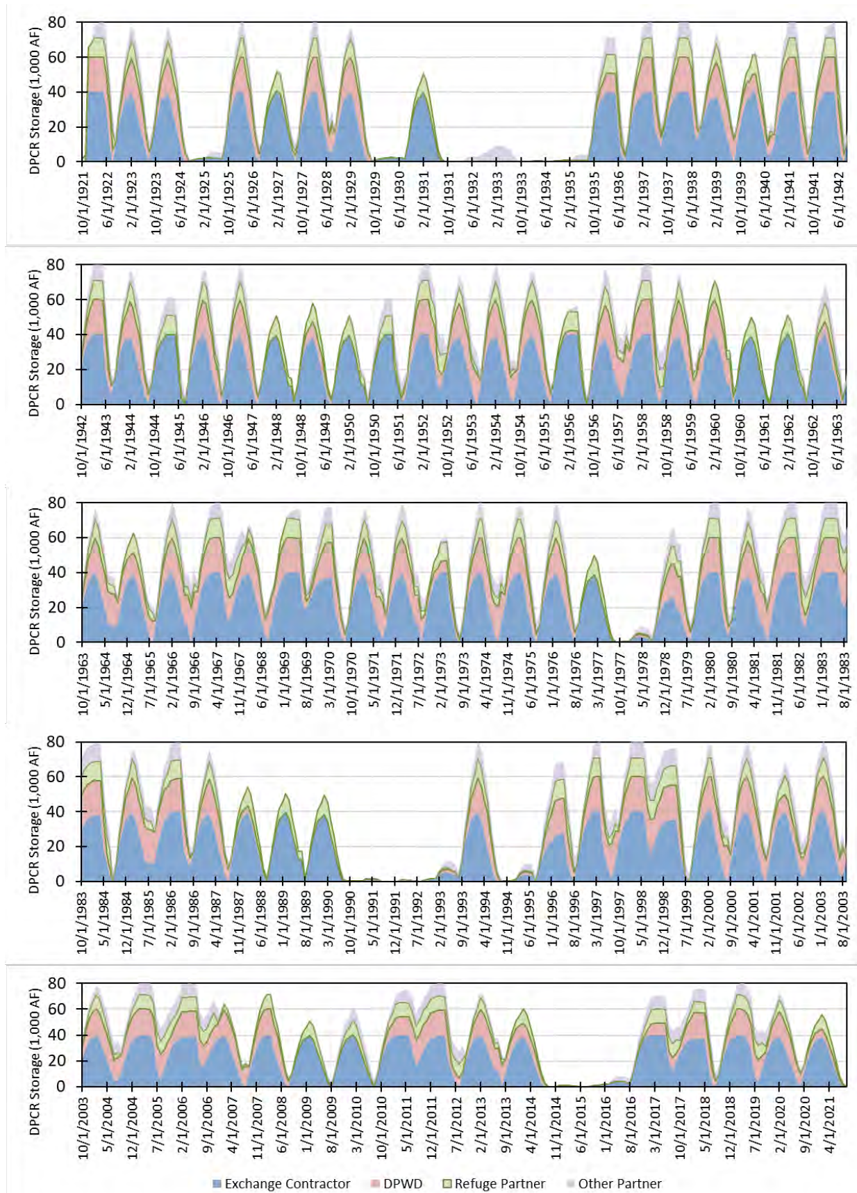
Figure 4. Combined DPCR Storage Timeseries [PA]
