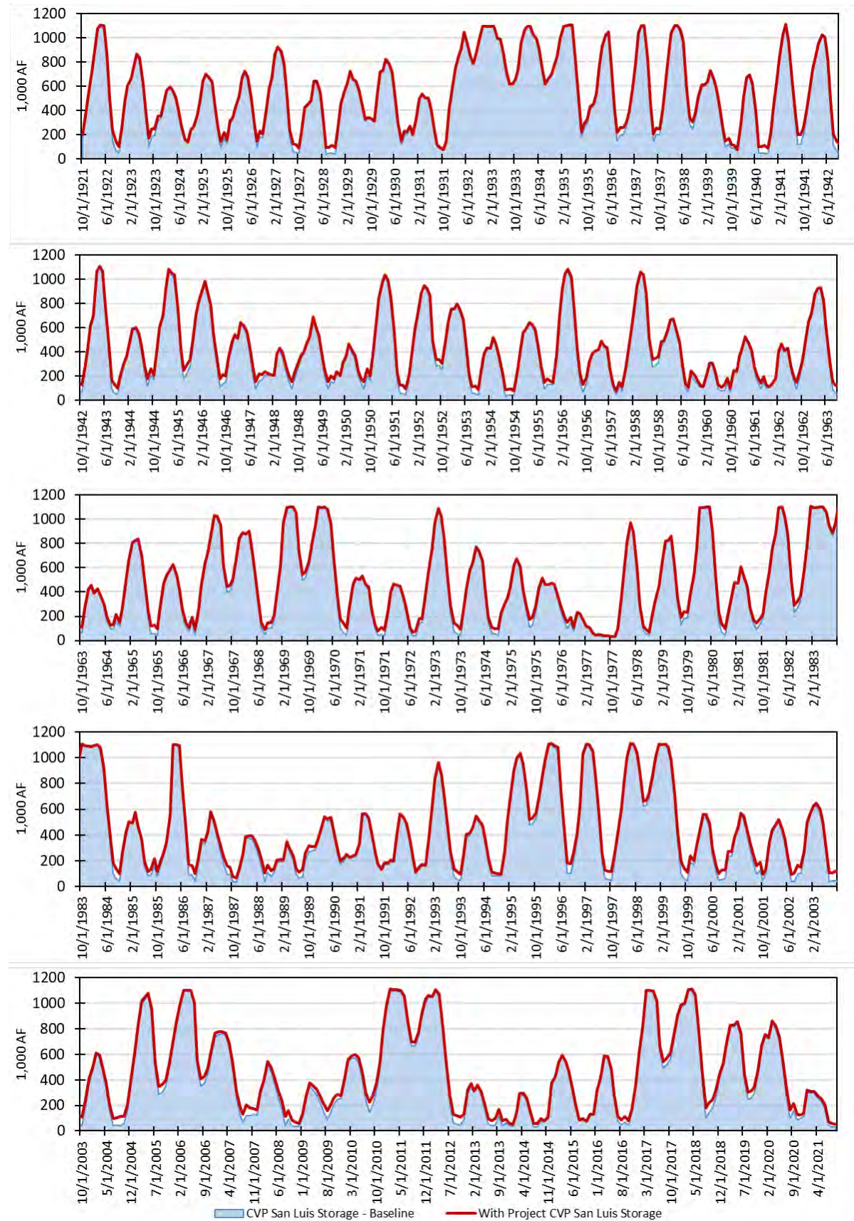
Figure 6. CVP San Luis Reservoir Storage Under the Baseline and With Project [PA]
