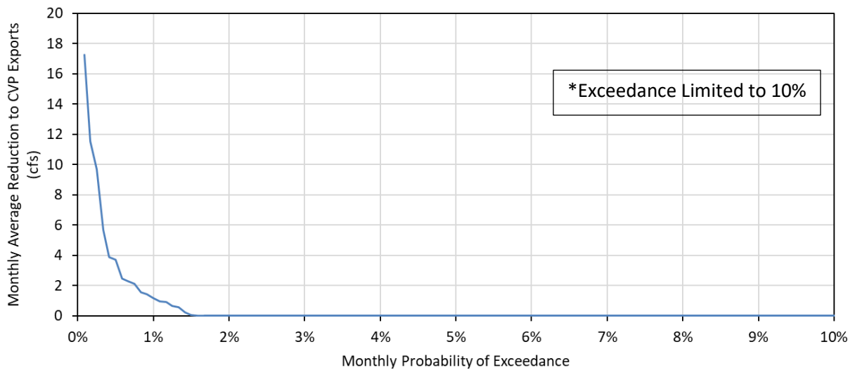
Figure 10. Monthly Probability of Exceedance (1,200 months) of Potential Reduction to CVP Exports from Changed Del Puerto Creek Flow [PA]
