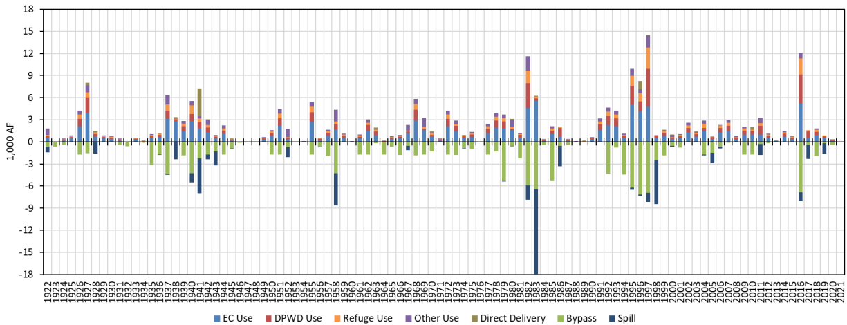
Figure 5. Annual Disposition of Del Puerto Creek Inflow [PA]
