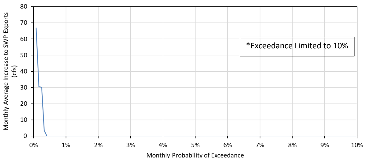
Figure 12. Monthly Probability of Exceedance (1,200 months) of Increases to SWP Exports from Potential CVP Foregone Pumping [PA]
