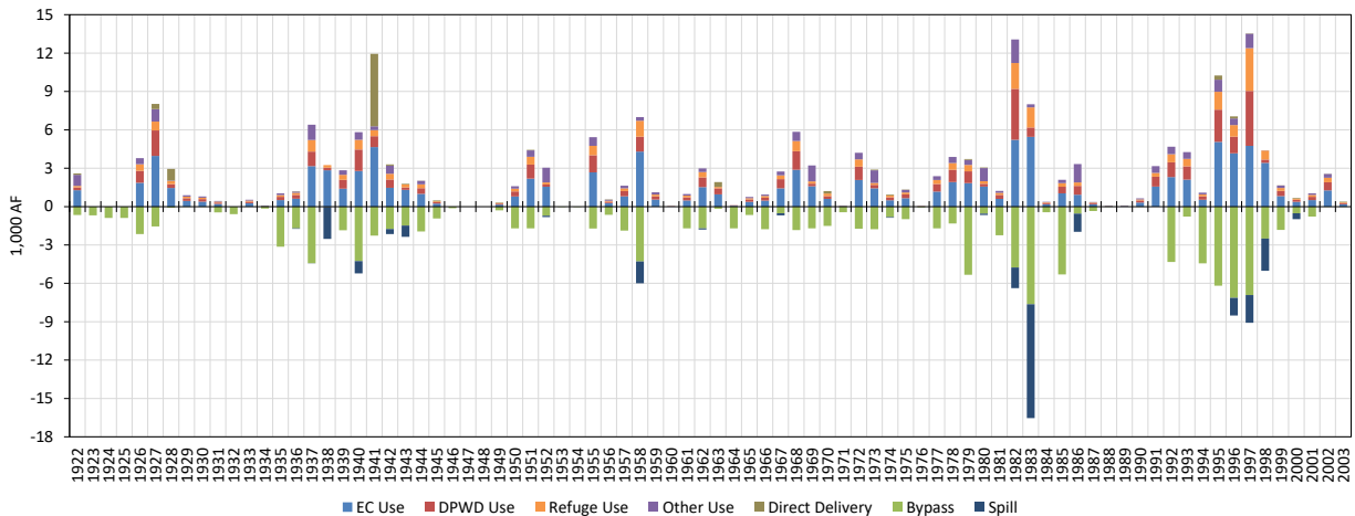
Figure 4. Annual Disposition of Del Puerto Creek Inflow
