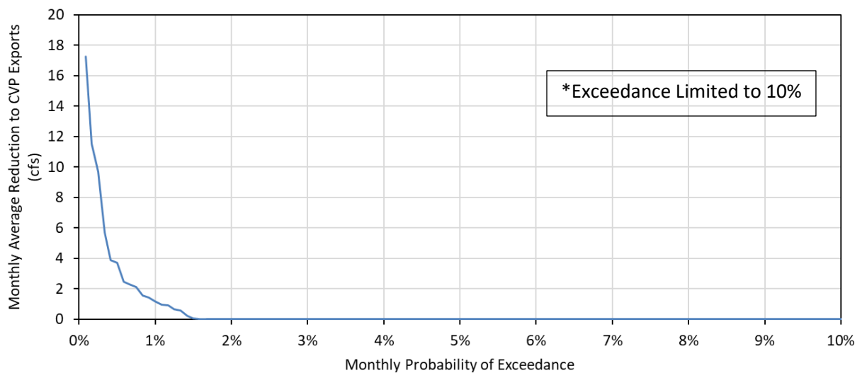
Figure 7. Monthly Probability of Exceedance (1,200 months) of Potential Reduction to CVP Exports from Changed Del Puerto Creek Flow [NAA]
