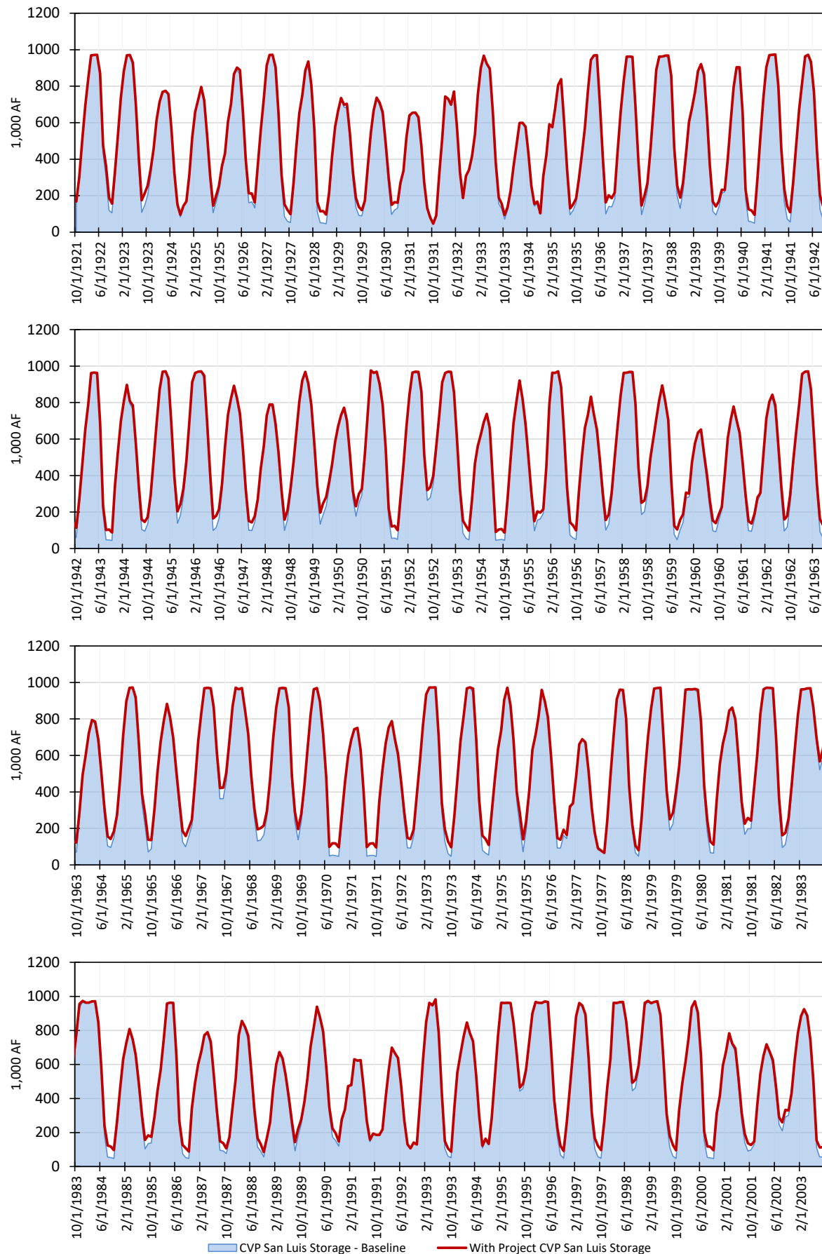
Figure 5. CVP San Luis Reservoir Storage Under the Baseline and With Project
