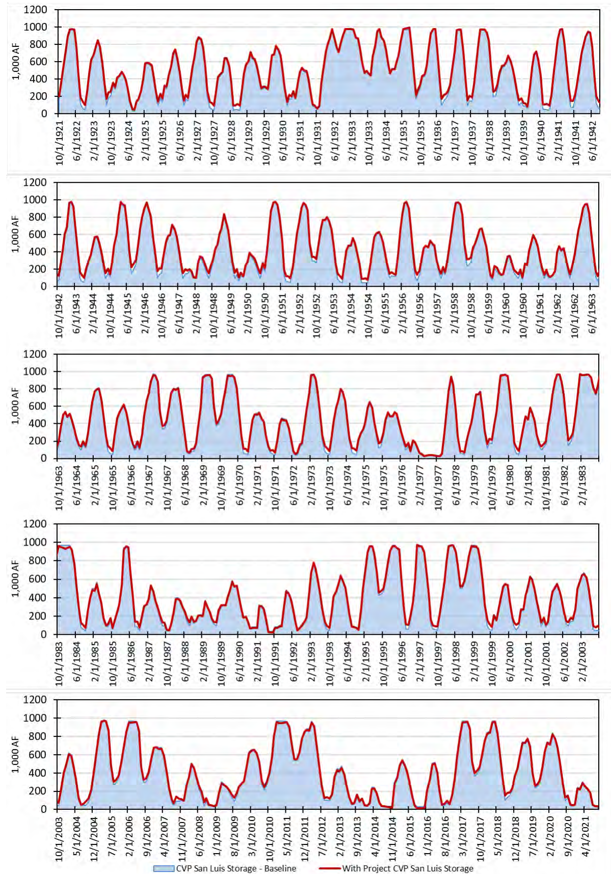
Figure 3. CVP San Luis Reservoir Storage Under the Baseline and With Project [NAA]
